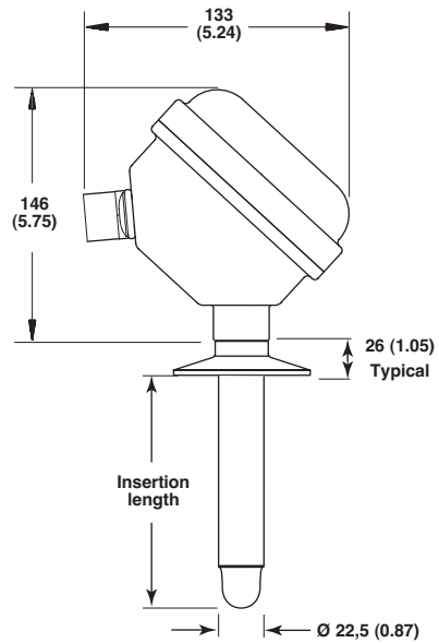
Model TD2 Integral electronics with TMA Spherical Tip Sensor
