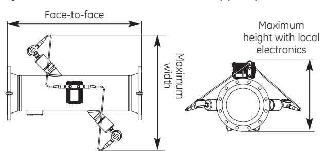
Design Reference C: 6 in to 24 in (150 mm to 600 mm) pipes, 1 path
