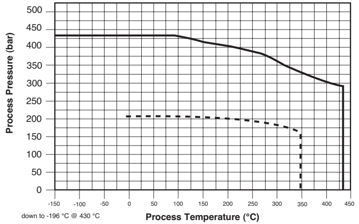
— 7MD GWR probe
