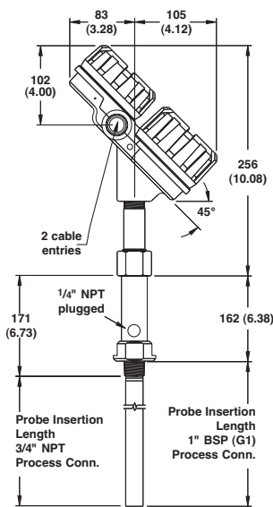
7MM / 7MN with flushing connection
