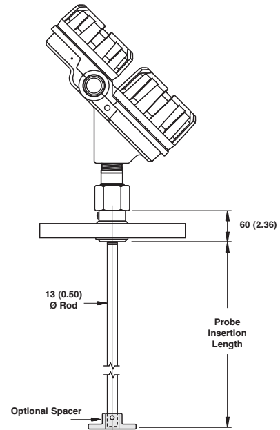
7MF/7MJ with flanged connection max. 6 m (240")
