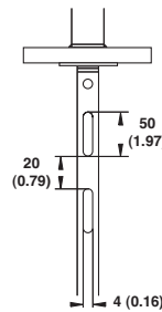
Slots for 7MR-A (order per “x” description)
