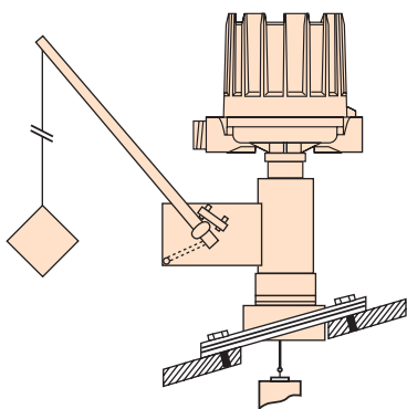
TYPICAL PROOF-ER INSTALLATION WITH VERSA FLANGE
