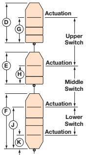
Model C10 Displacer Arrangement E
