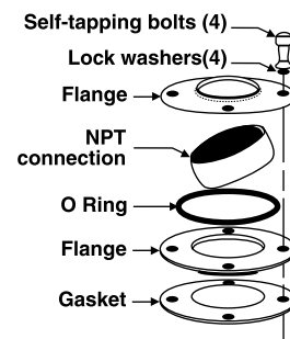
VERSA FLANGE ASSEMBLY PART NUMBER 089-5207-001
