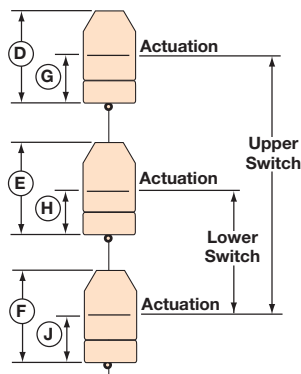
Model B10 Displacer Arrangement 4
