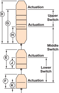
Model C10 Displacer Arrangement F
