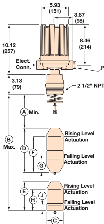
Model B15 with Threaded Mounting
