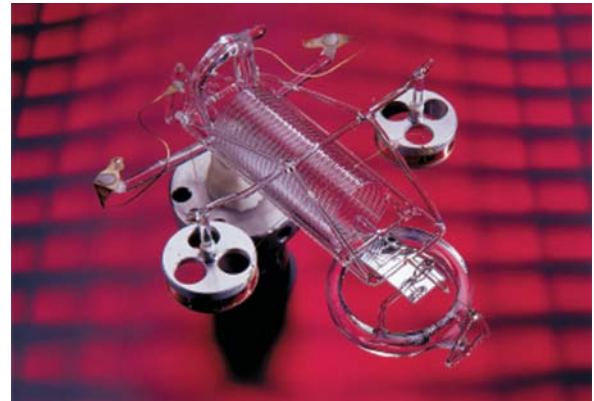
The Series 7250 features GE's unique fused-quartz sensor. This rugged transducer offers unequalled precision and a stability of 0.0075% of reading per year.
