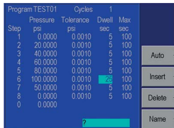
All Series 7250s are fully programmable and can store up to 20 separate programs with up to 1000 steps.
